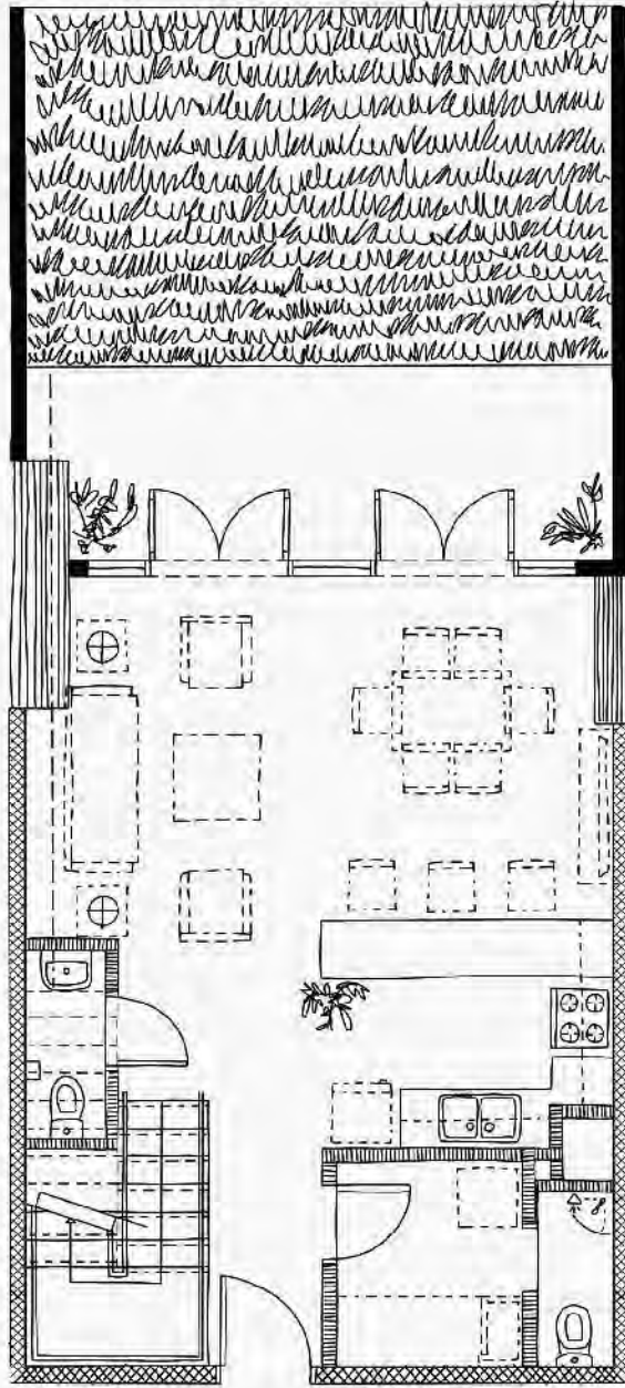
Garden Unit Level 01
