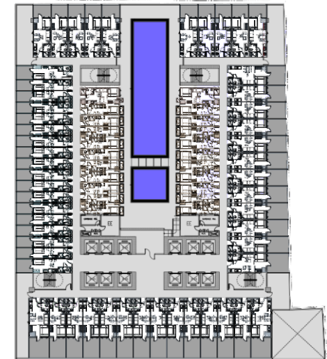
Typical 8th Floor Plan (Amenities Floor)
