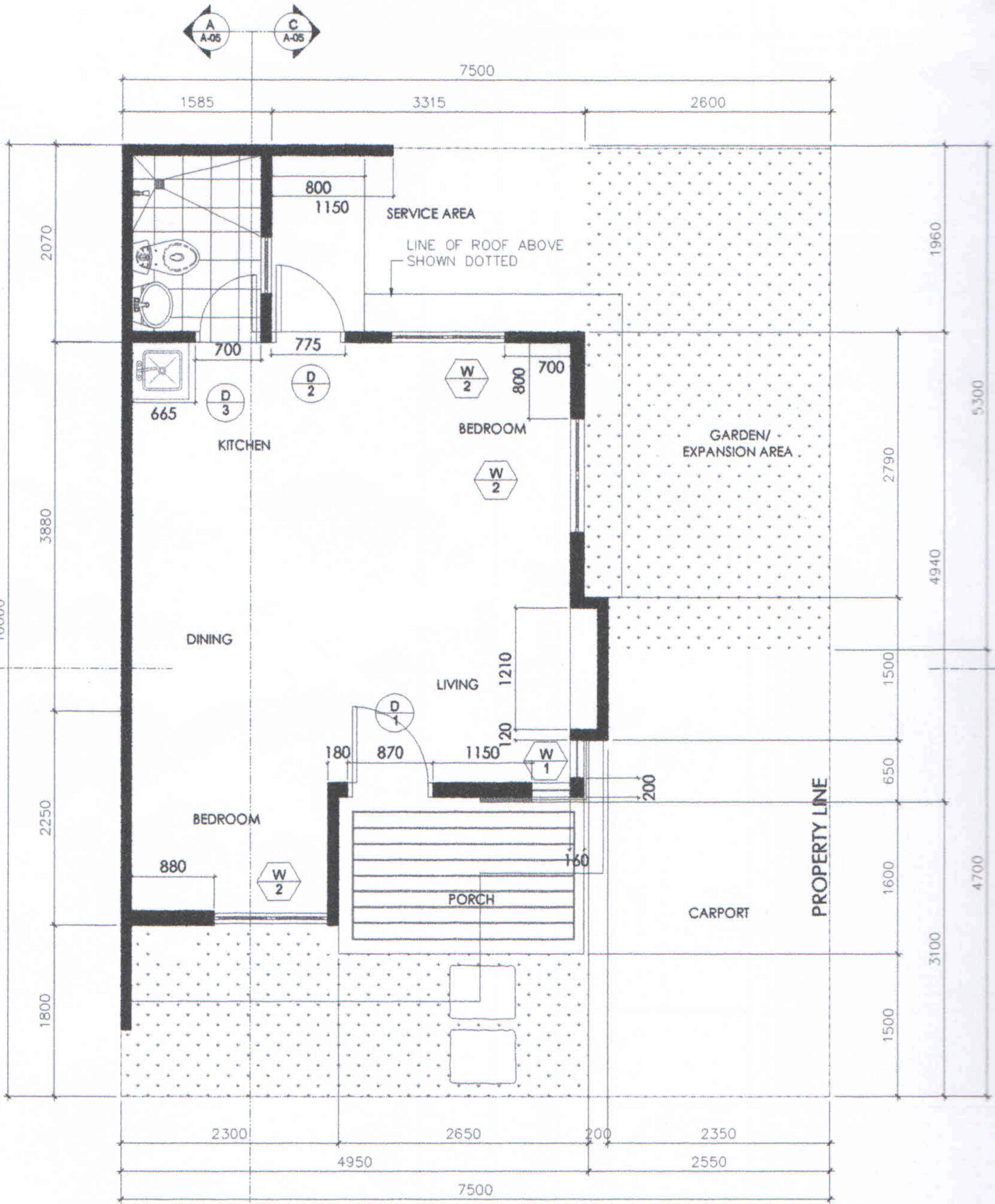
1 FLOOR PLAN A-02 SCALE 1:50
