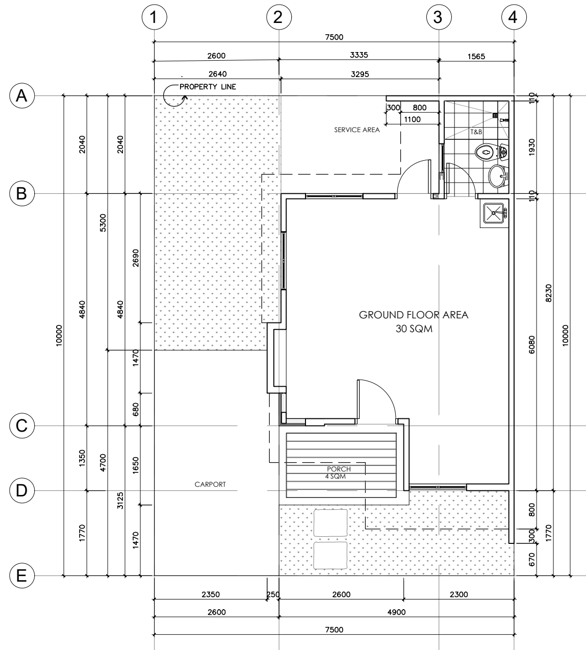
1 GROUND FLOOR PLAN --- SCALE 1:80 MTS
