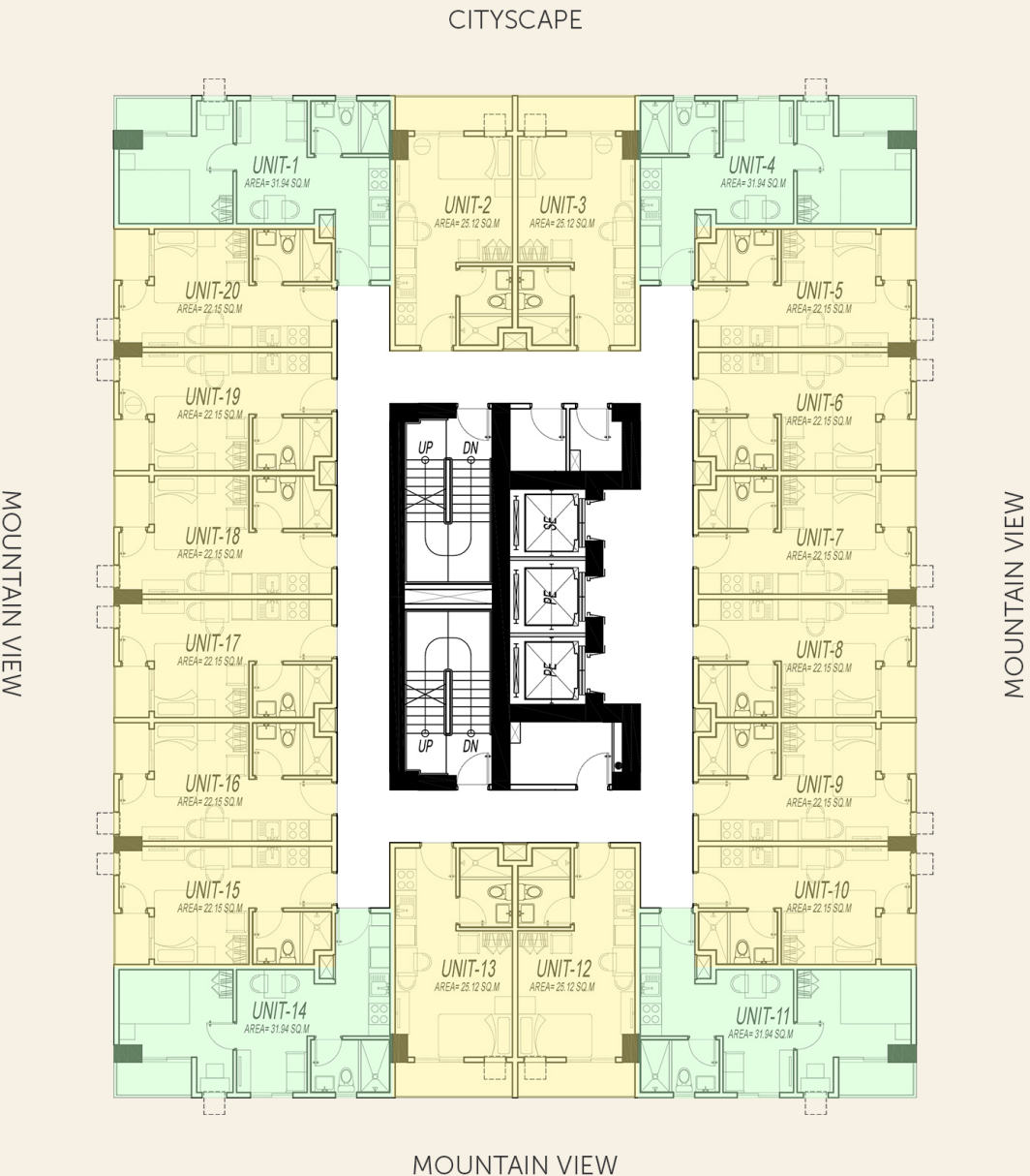
6th - 21st Level Floor Plan
