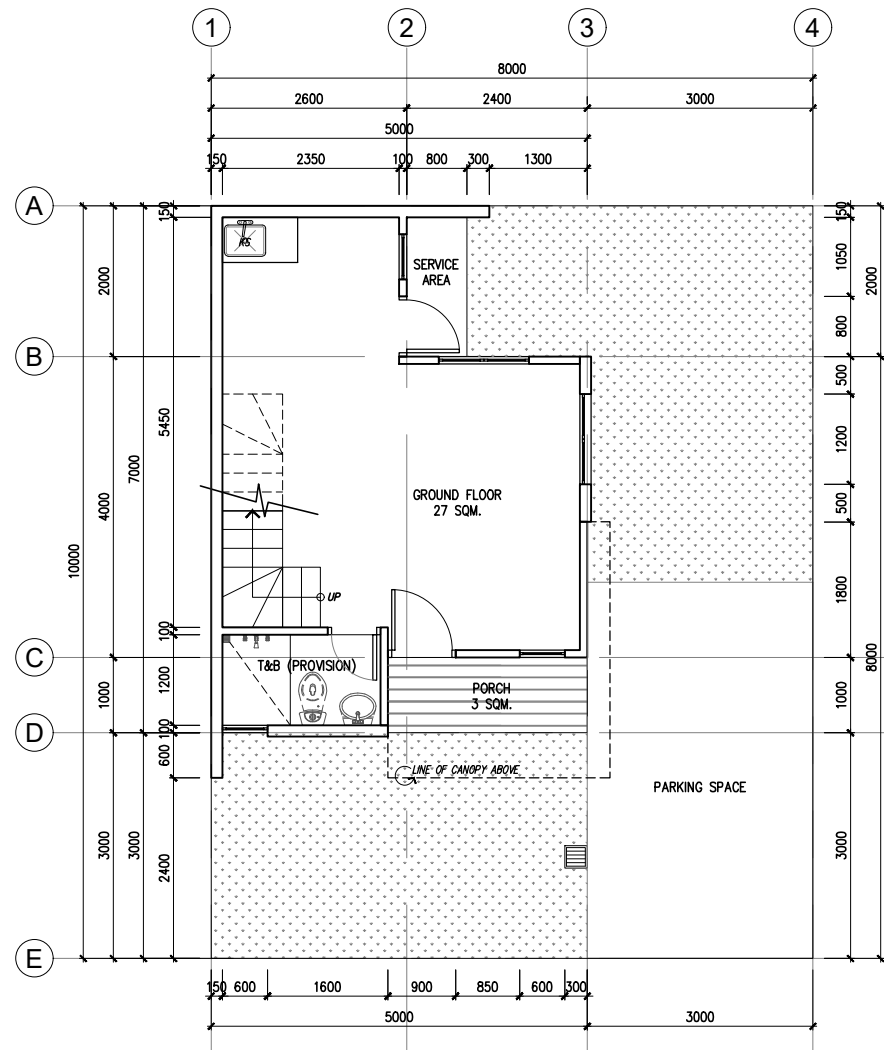
1 GROUND FLOOR PLAN --- SCALE 1:100 MTS
