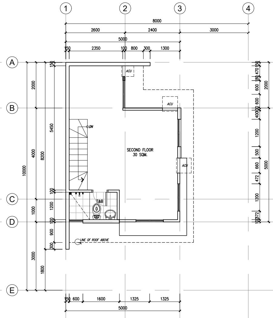
2 SECOND FLOOR PLAN --- SCALE 1:100 MTS
