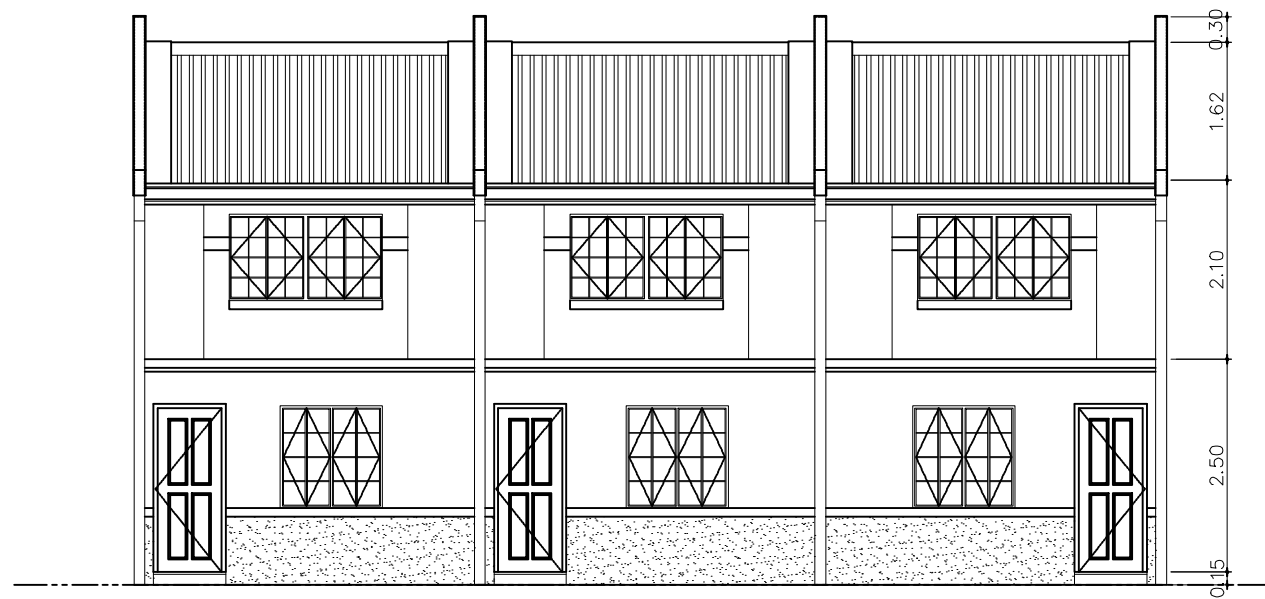
FRONT ELEVATION
