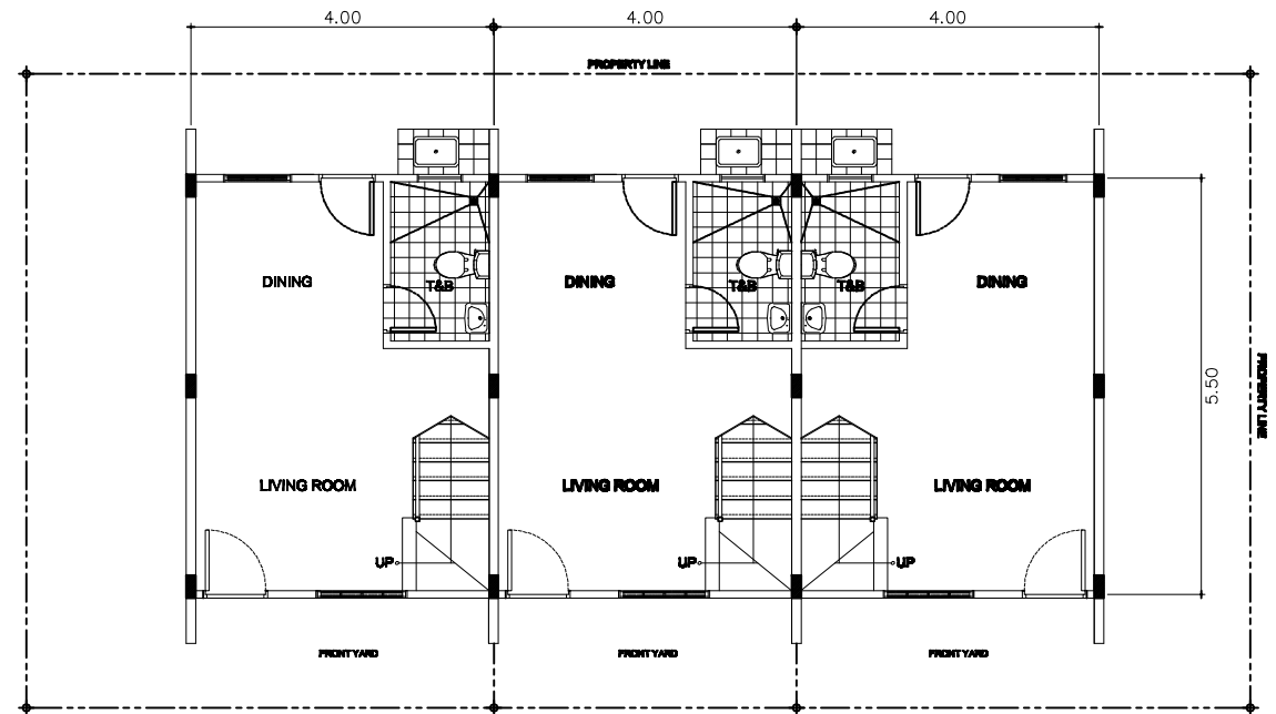
TYPICAL GROUND FLOOR PLAN
