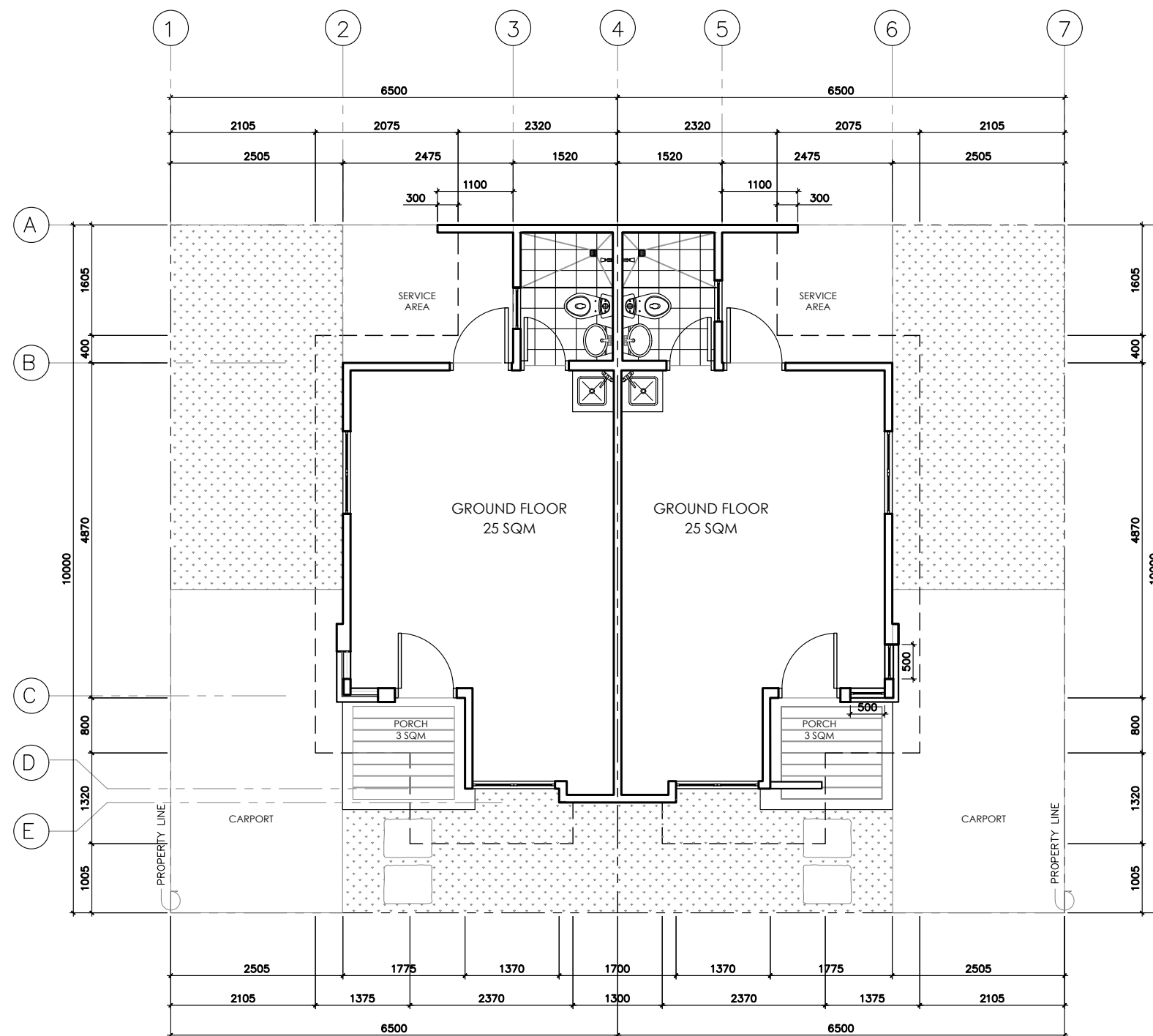
1 GROUND FLOOR PLAN -- SCALE 1:80 MTS
