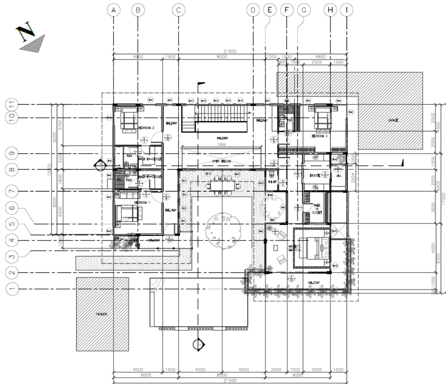
A SECOND FLOOR PLAN 3 | 1 SCALE 1:100 MTS
